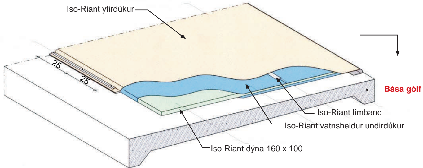
Isometry
