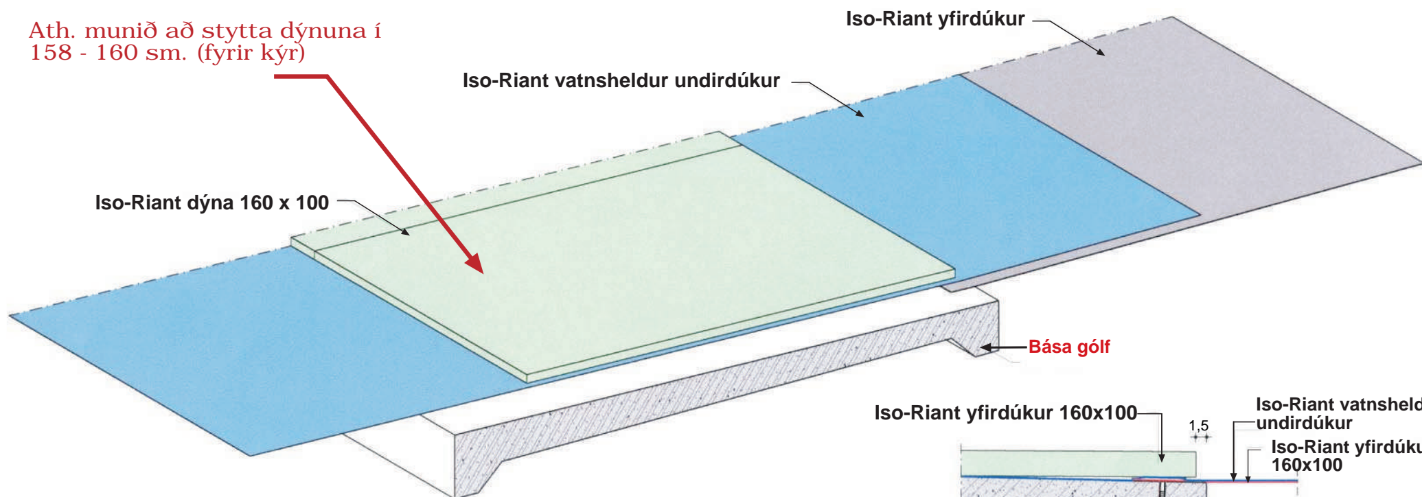
Isometry
